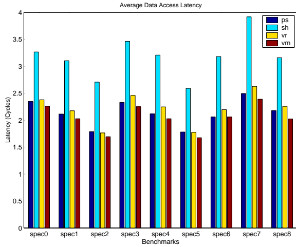
Figure 15. Access latencies of multi-programmed workloads. Configuration 1: 8+8/256/16FO4.
